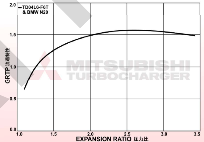
TURBINE MAP
