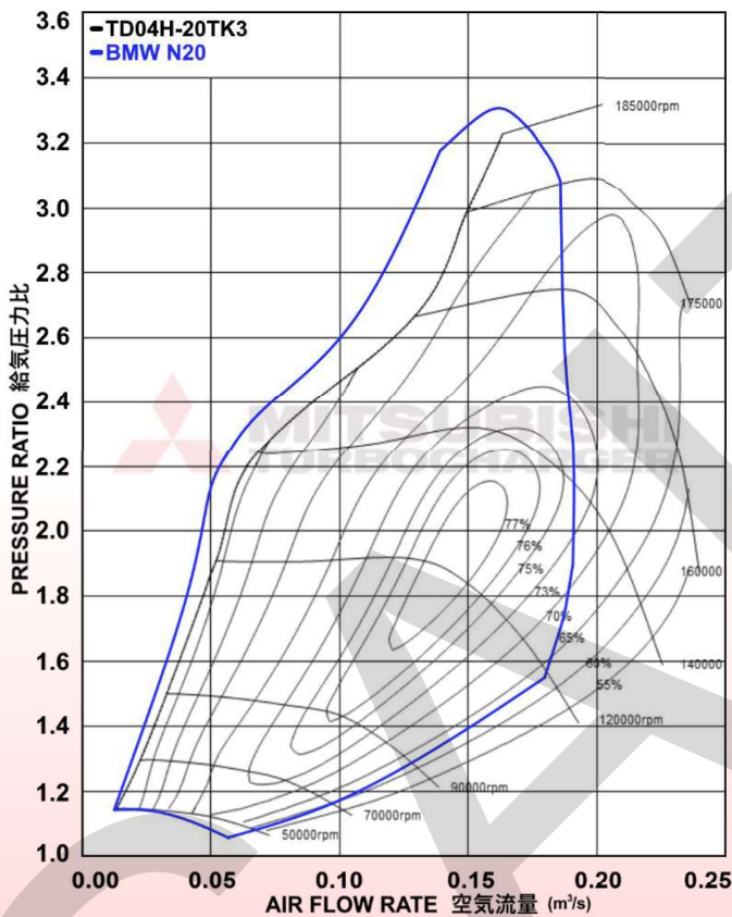
COMPRESSOR MAP
