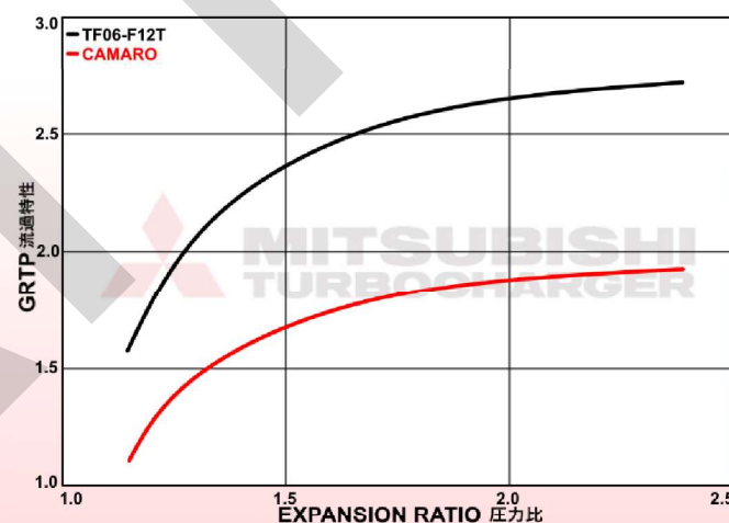
TURBINE MAP
