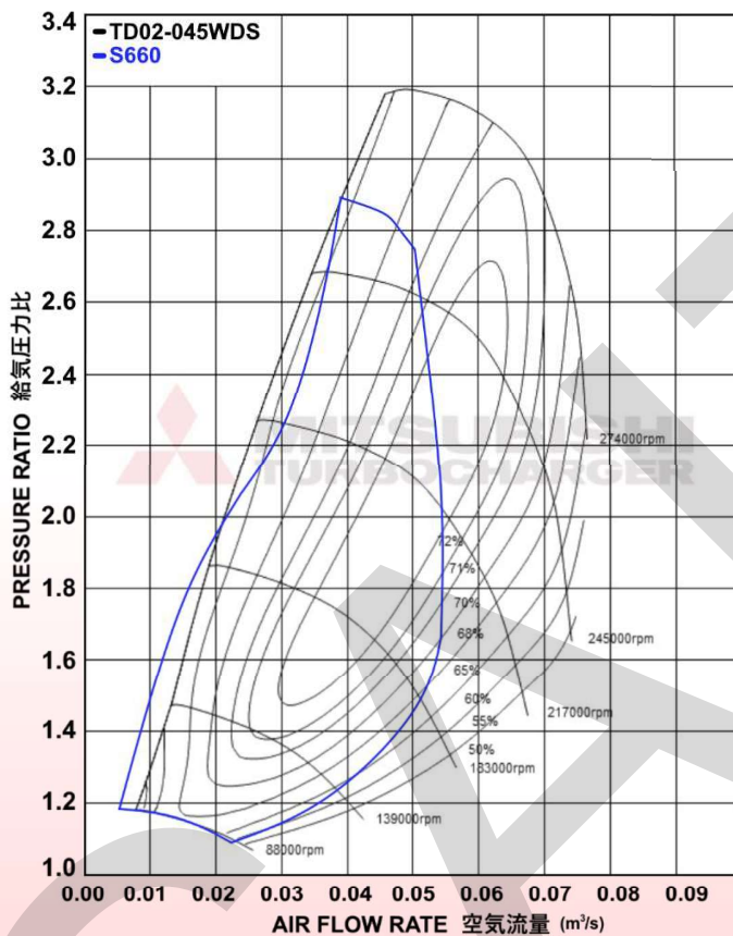
COMPRESSOR MAP
