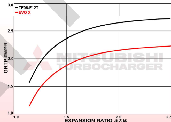
TURBINE MAP
