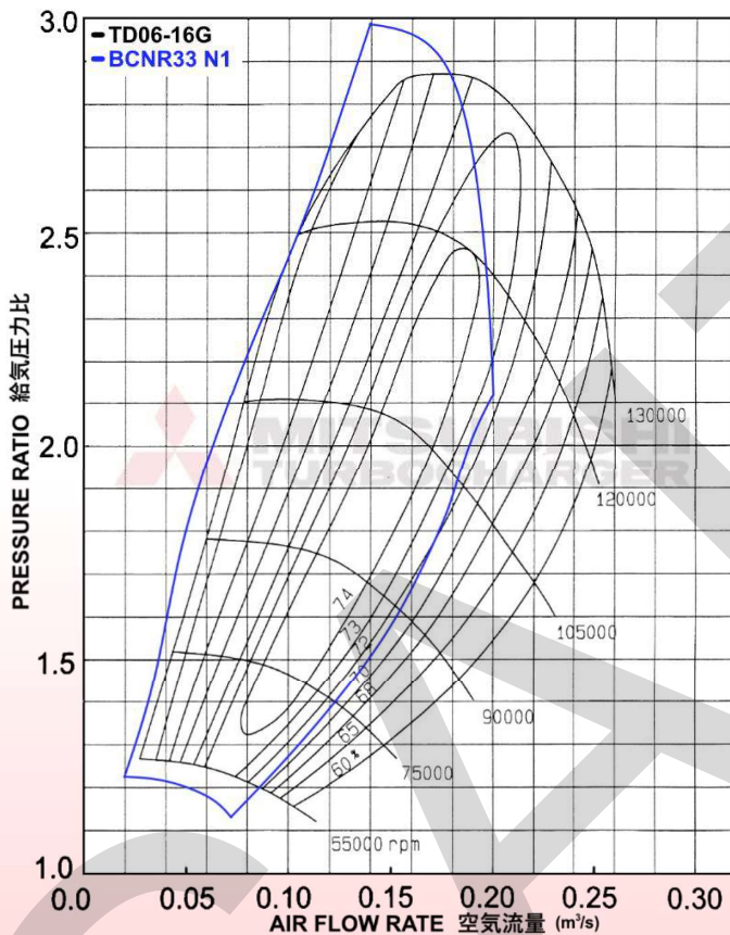
COMPRESSOR MAP
