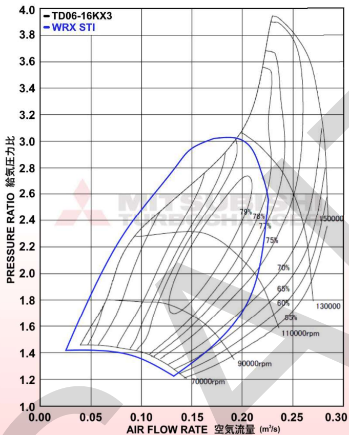
COMPRESSOR MAP
