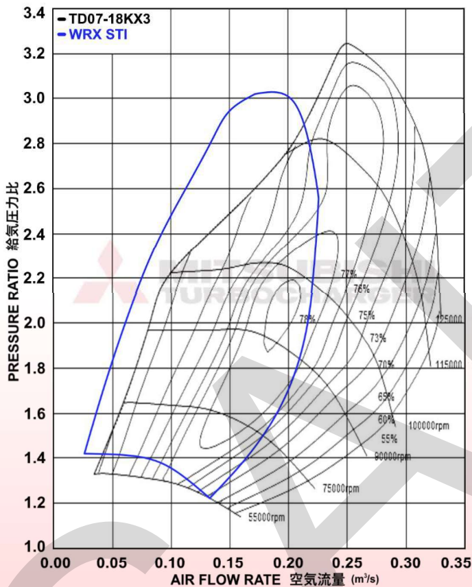
COMPRESSOR MAP
