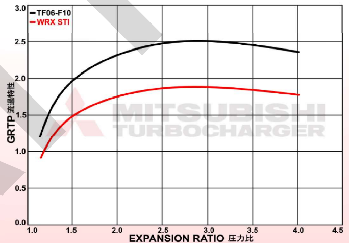
TURBINE MAP
