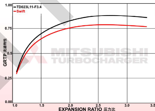
TURBINE MAP
