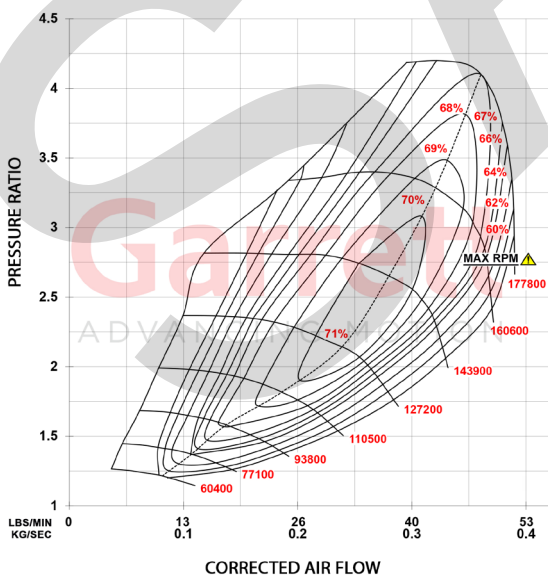
Compressor Map
